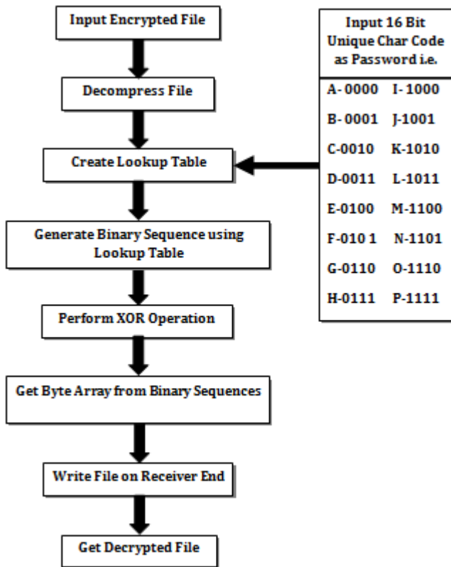
Figure 4: Decryption Process
