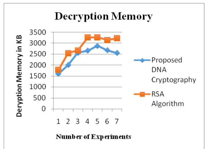
Figure 8: Decryption Memory
