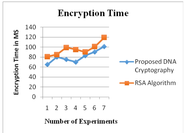
Figure 5: Encryption Time
