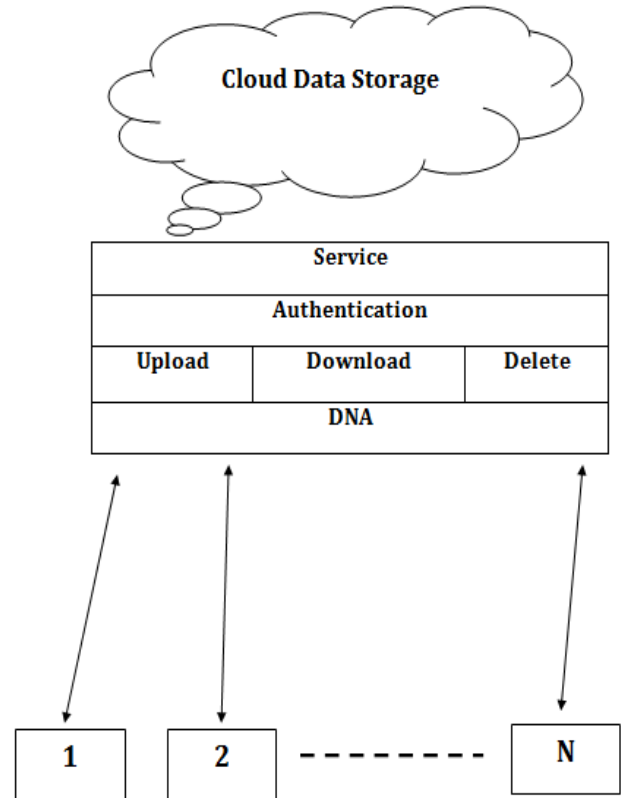
Figure 2: Proposed Systems
