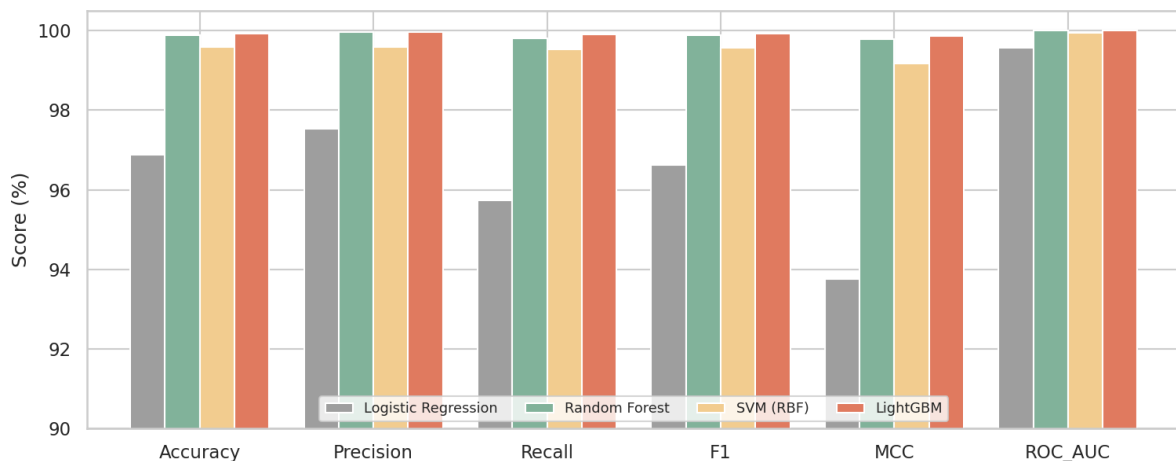
Figure 4. Classification metrics of the four models on the test set
