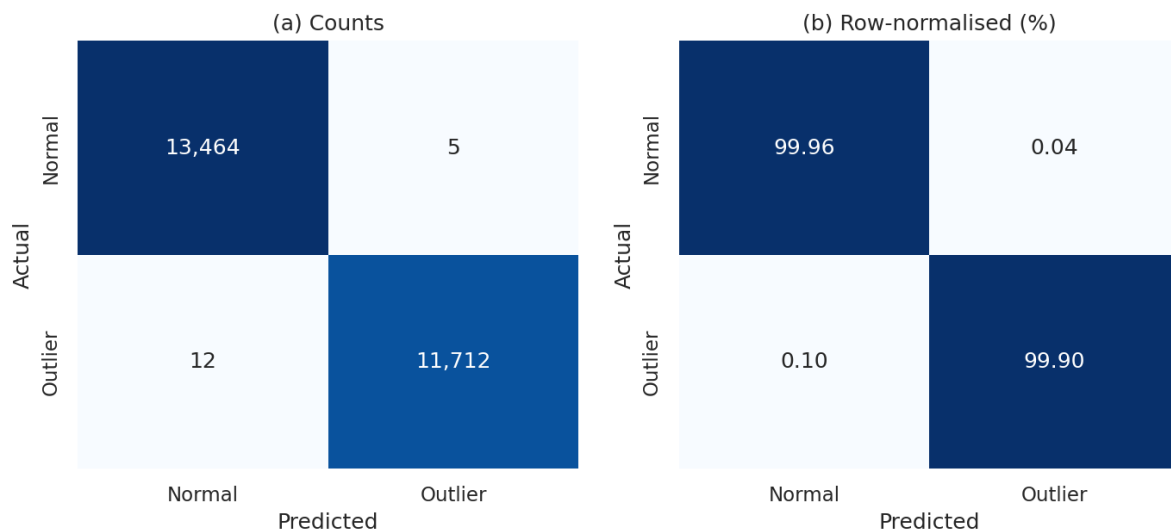
Figure 1. Confusion matrix of LightGBM on the test set: (a) counts and (b) row-normalised percentages
