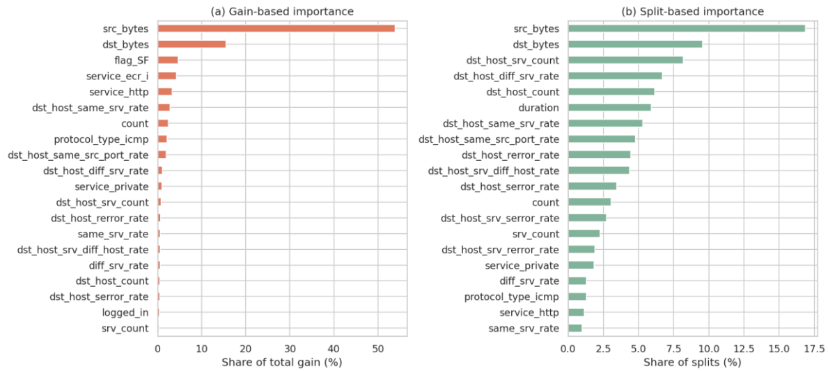
Figure 3. LightGBM feature importance by (a) information gain and (b) split frequency
