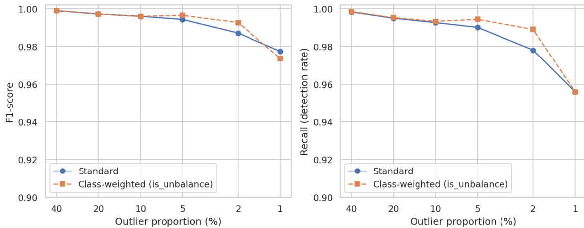
Figure 5. F1-score (a) and recall (b) of LightGBM as the outlier proportion decreases
