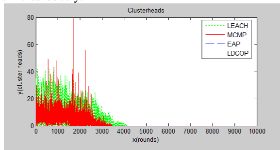
Figure 2: Cluster Head selection using LEACH and low duty cycle optimization protocol using multilevel clustering(LDCOP)
